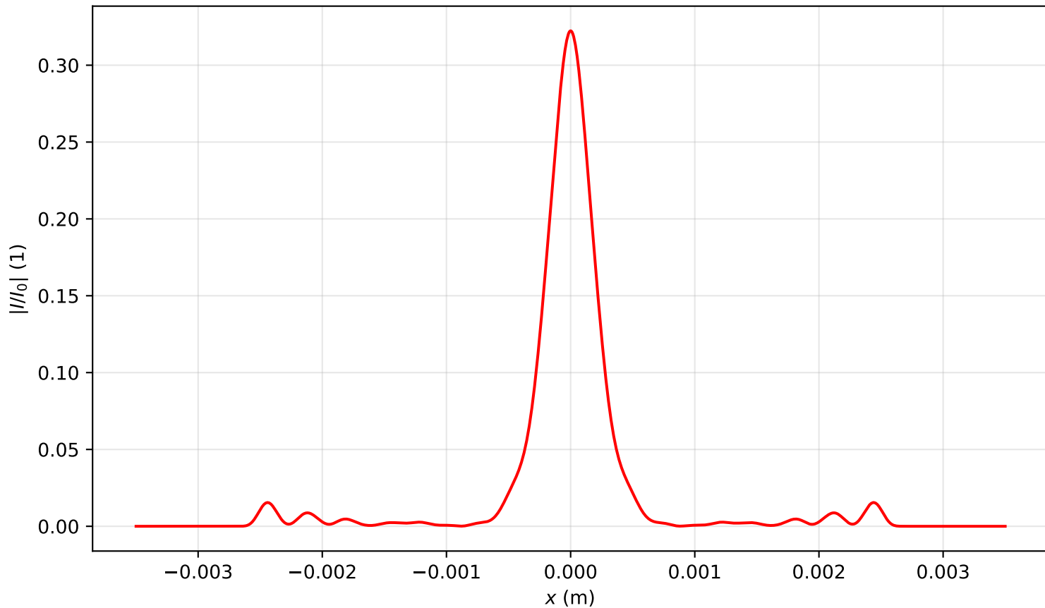
Intensity profile I(x, y = 0, z = 2.070)/I_0 , P_{in}=6.0P_{cr} , artificial time
